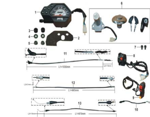
B10 = 仪表、钢索、锁具和开关 / METER, CABLES, LOCKS & SWITCH / VELOCIMETRO, GUAYAS Y CERRADURAS
