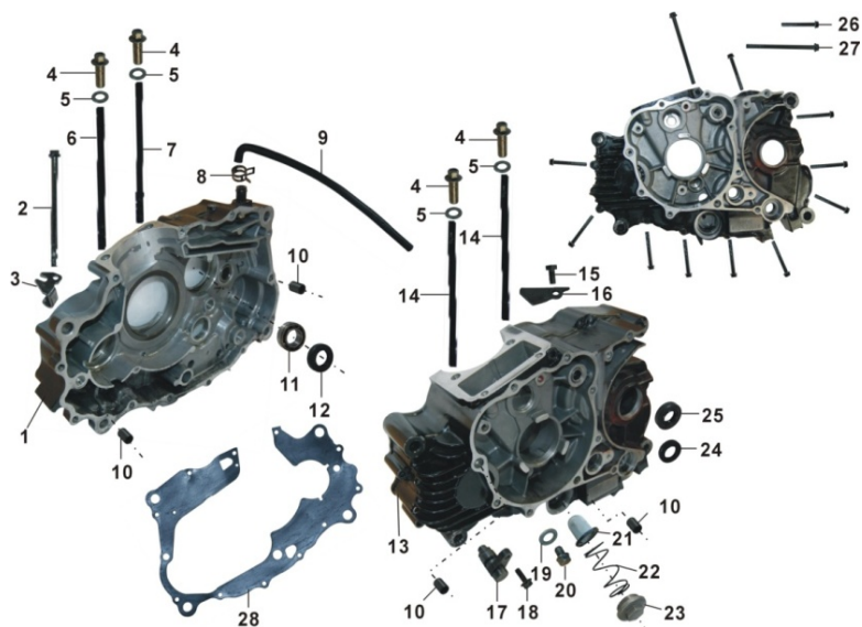
E04 = 曲轴箱 / CRANKCASE ASSEMBLY / CARCAZAS DE MOTOR (CARTER)
