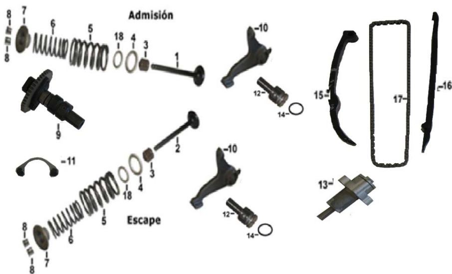
E01 = 进气和排气系统 / AIR INLET EXHAUST SYSTEM / TREN DE VALVULAS
