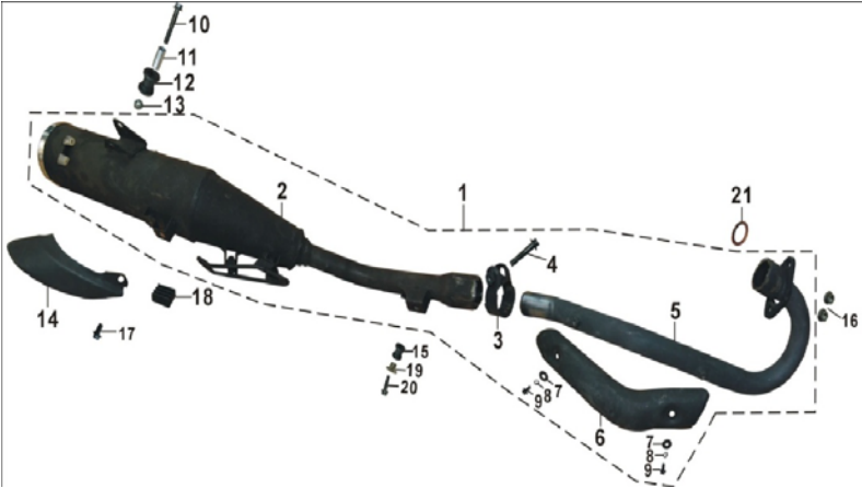
B11 = 消声器 / MUFFLER ASSY / ESCAPE
