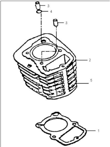
E06 = 汽缸体 / CYLINDER BLOCK / CILINDRO DE MOTOR
