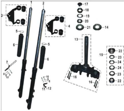
B17 = 方向柱、前减 / STEERING STEM, FRONT SHOCK ABSORBER / SUSPENSION DELANTERA
