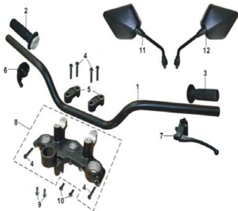
B08 = 方向把 / HANDLE BAR / MANUBRIO
